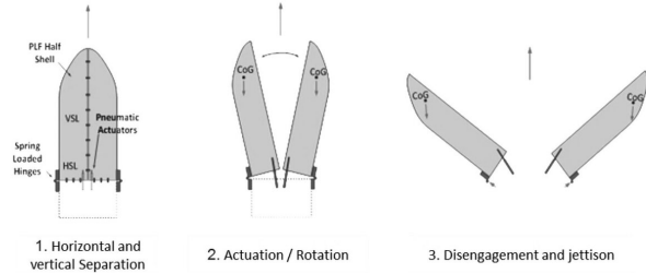
Figure 7: Separation of fairings
