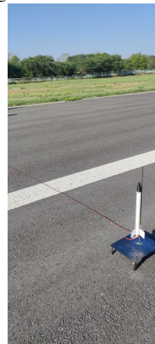
Figure: 67 Launch Setup
