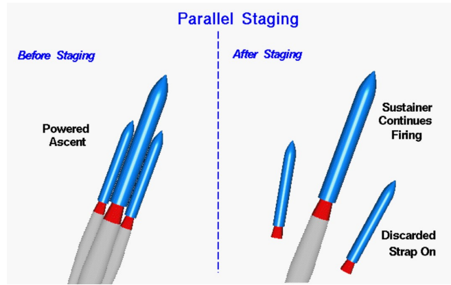
Figure 13: Parallel Staging
