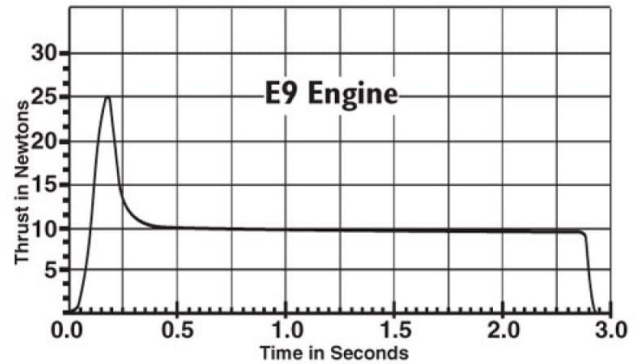
Figure: 60 Thrust vs Time graph
