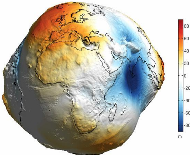
Figure 40: Non Spherical Earth
