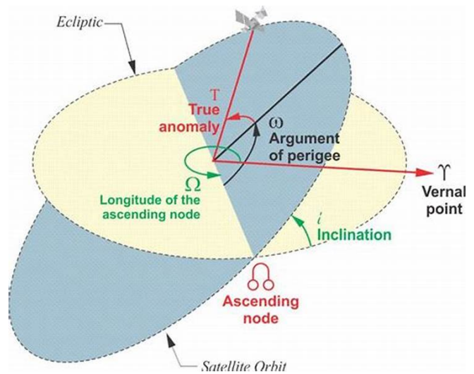
Figure 36: Keplerian elements
