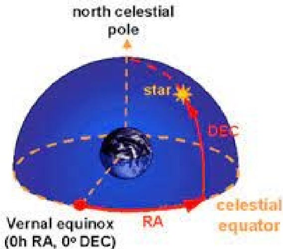
Figure 33: Outline of the RA-Dec Coordinate System
