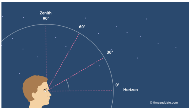
Figure 31 Altitude: Angle made by object with horizon
