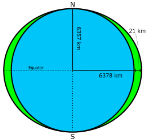
Figure 42: Oblate Earth
