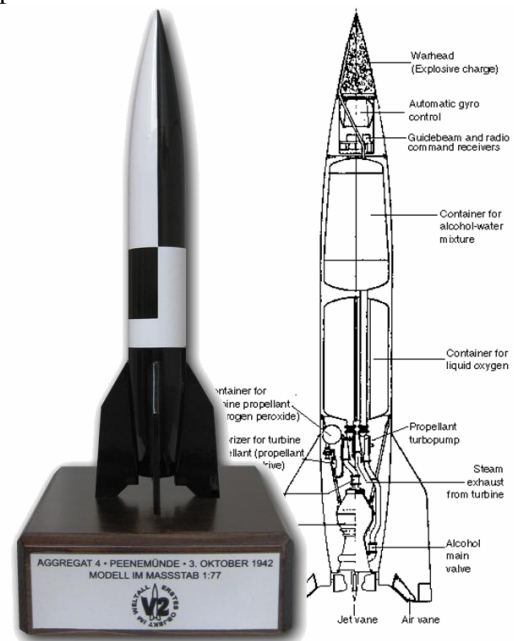
Figure 2: V2 Rocket
