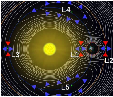
Figure 37: Lagrange points
