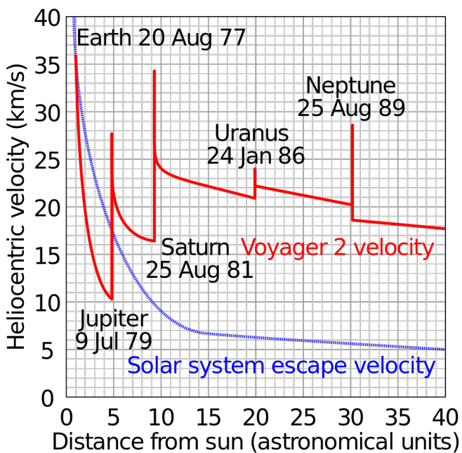
Figure 48: Voyager 2 speed
