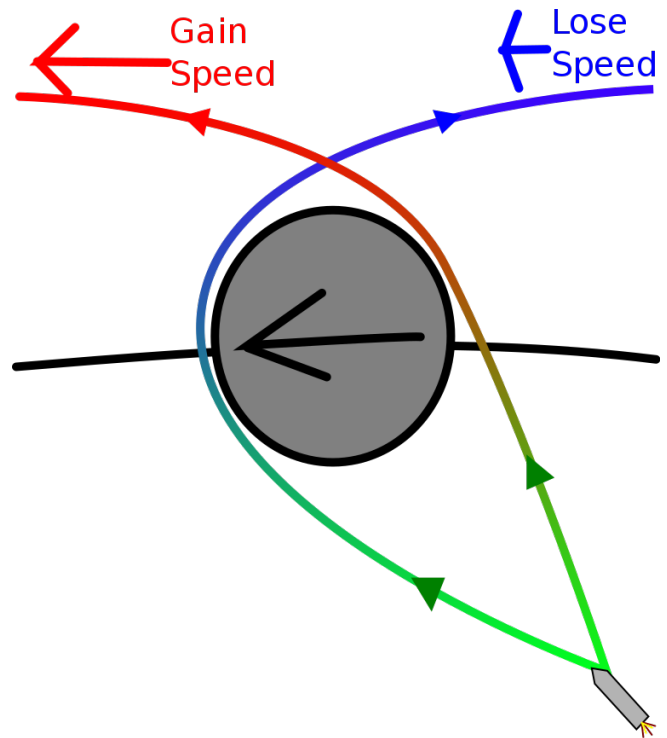
Figure 46: Gravitational Assist
