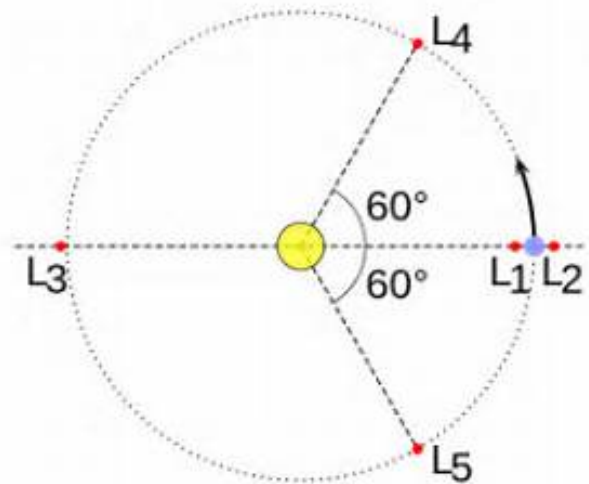
Figure 39: Lagrange points
