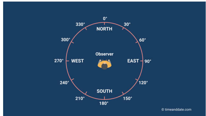
Figure 32: Azimuth: representing the object's cardinal direction
