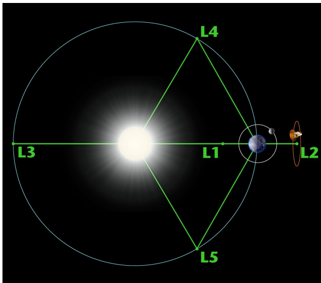
Figure 38: Lagrangian point of a two-body system
