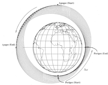
Figure 44: J2 Apsidal Rotation
