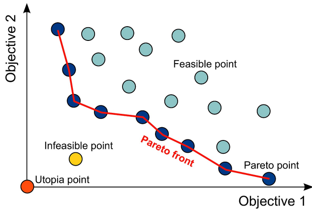
Figure 49: Pareto Front
