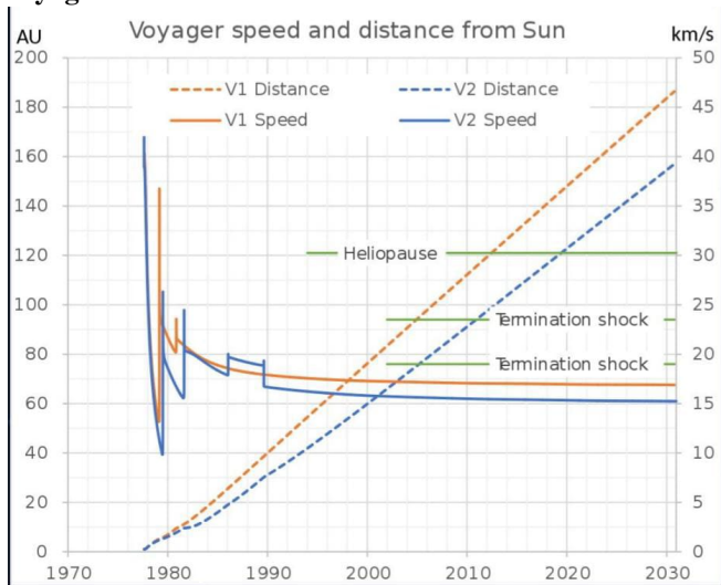
Figure 47: Voyager 1 and 2 speed
