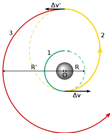
Figure 45: Hohmann Orbit Transfer
