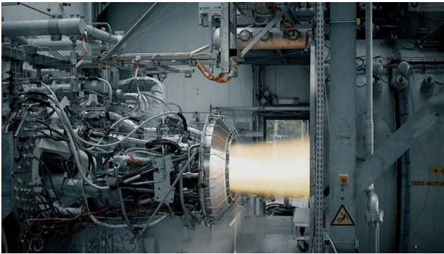
Figure 27: VINCI is a fresh attempt at a high performance Expander Cycle engine (ESA)
