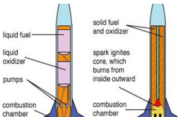
Figure 19: Cross section views of liquid- and solid-propellant rockets
