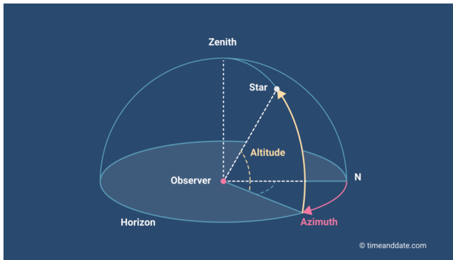
Figure 30: Upper hemisphere of the celestial sphere
