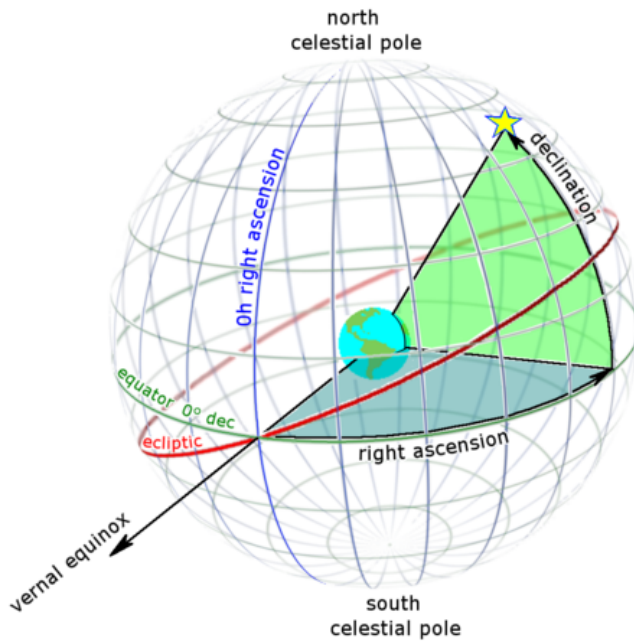
Figure 35: A nice demonstration of RA and Dec
