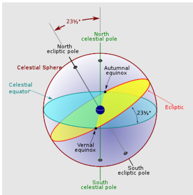
Figure 34: Celestial Sphere
