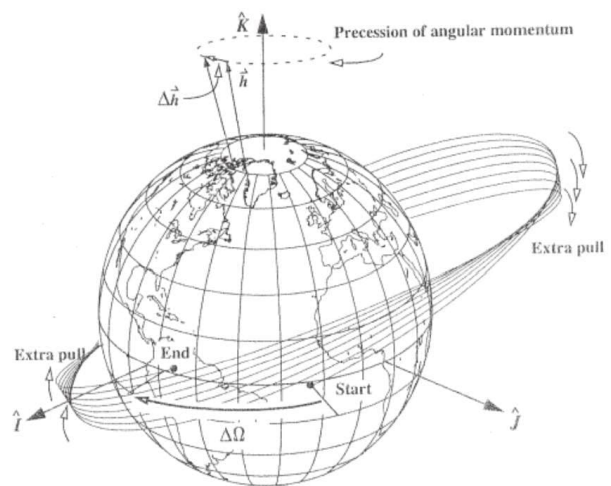
Figure 43: J2 Nodal Regression
