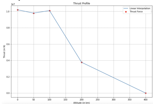
Graph of thrust vs altitude
